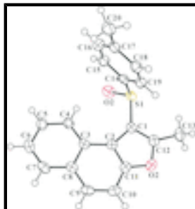
Fig. 1. The molecular structure of the title compound. Displacement ellipsoids are drawn at the 50% probability level.
