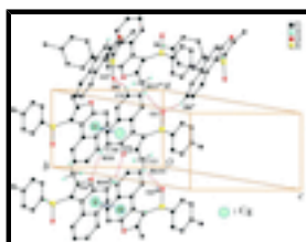
Fig. 2. A view of the C—H...O and \pi - \pi interactions (dotted lines) in the crystal structure of the title compound. H atoms non-participating in hydrogen-bonding were omitted for clarity. [Symmetry codes: (i) -x + 2, y + 1/2, -z + 1/2 ; (ii) -x, -y + 1, -z ; (iii) x - 1, y, z ; (iv) -x + 1, -y + 1, -z ; (v) -x + 2, y - 1/2, -z + 1/2 ; (vi) x + 1, y, z .]
